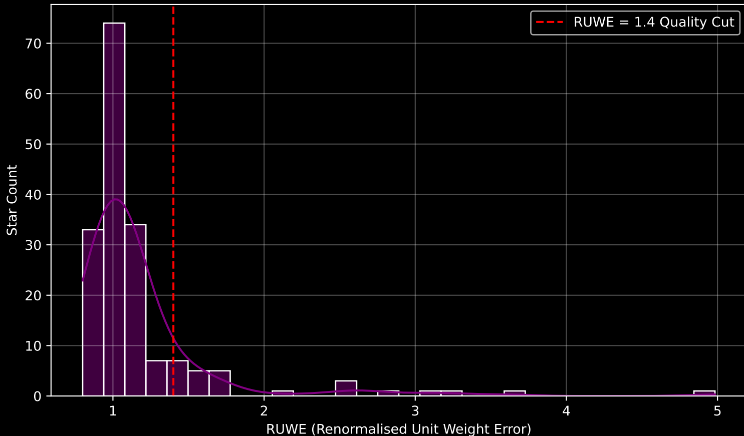
GAPOGEE DR17 Field [269-28-O_TESS] RUWE Distribution (n= 174)
