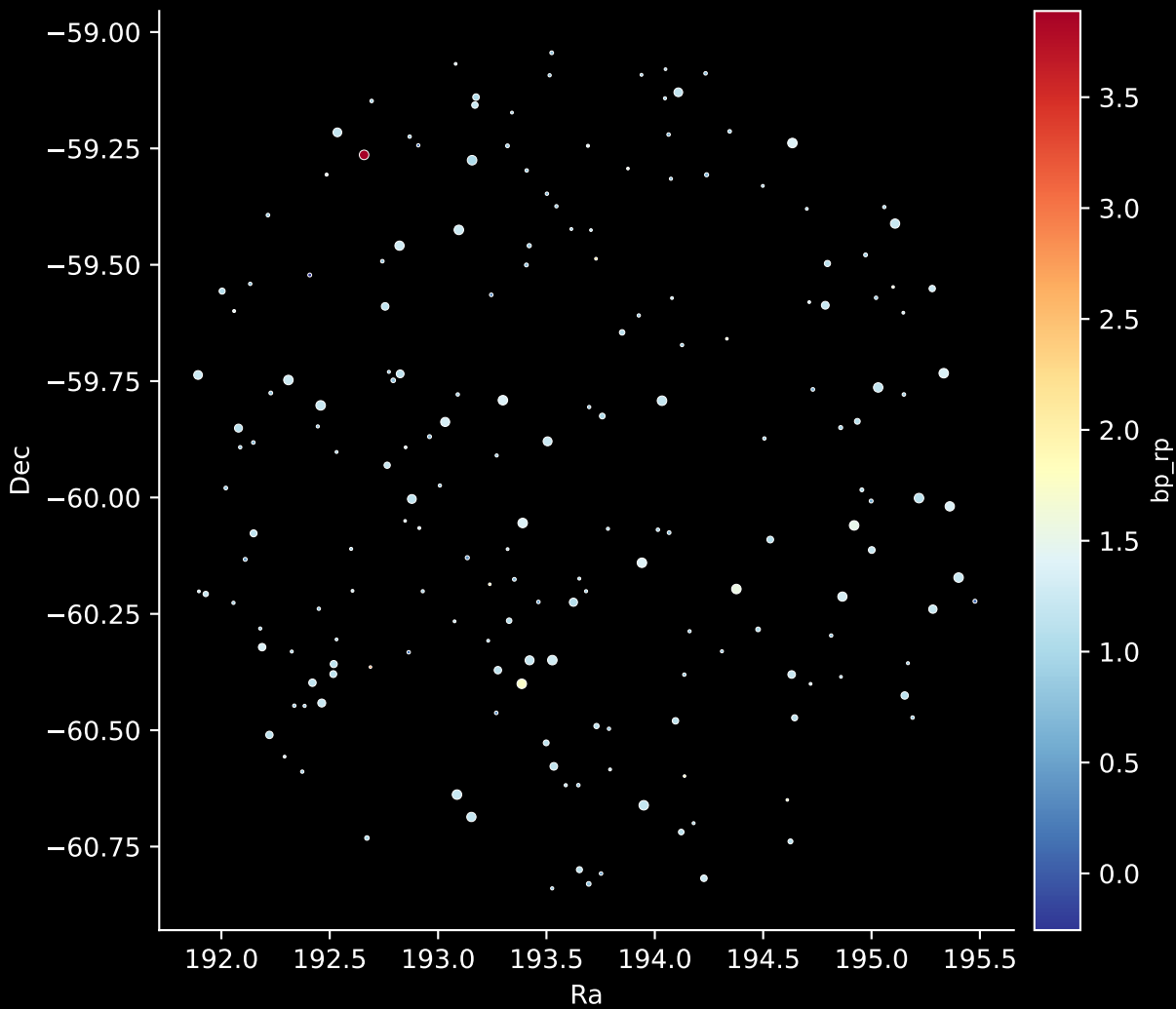
APOGEE DR17 Field: [269-28-O_TESS] Stars: 187
