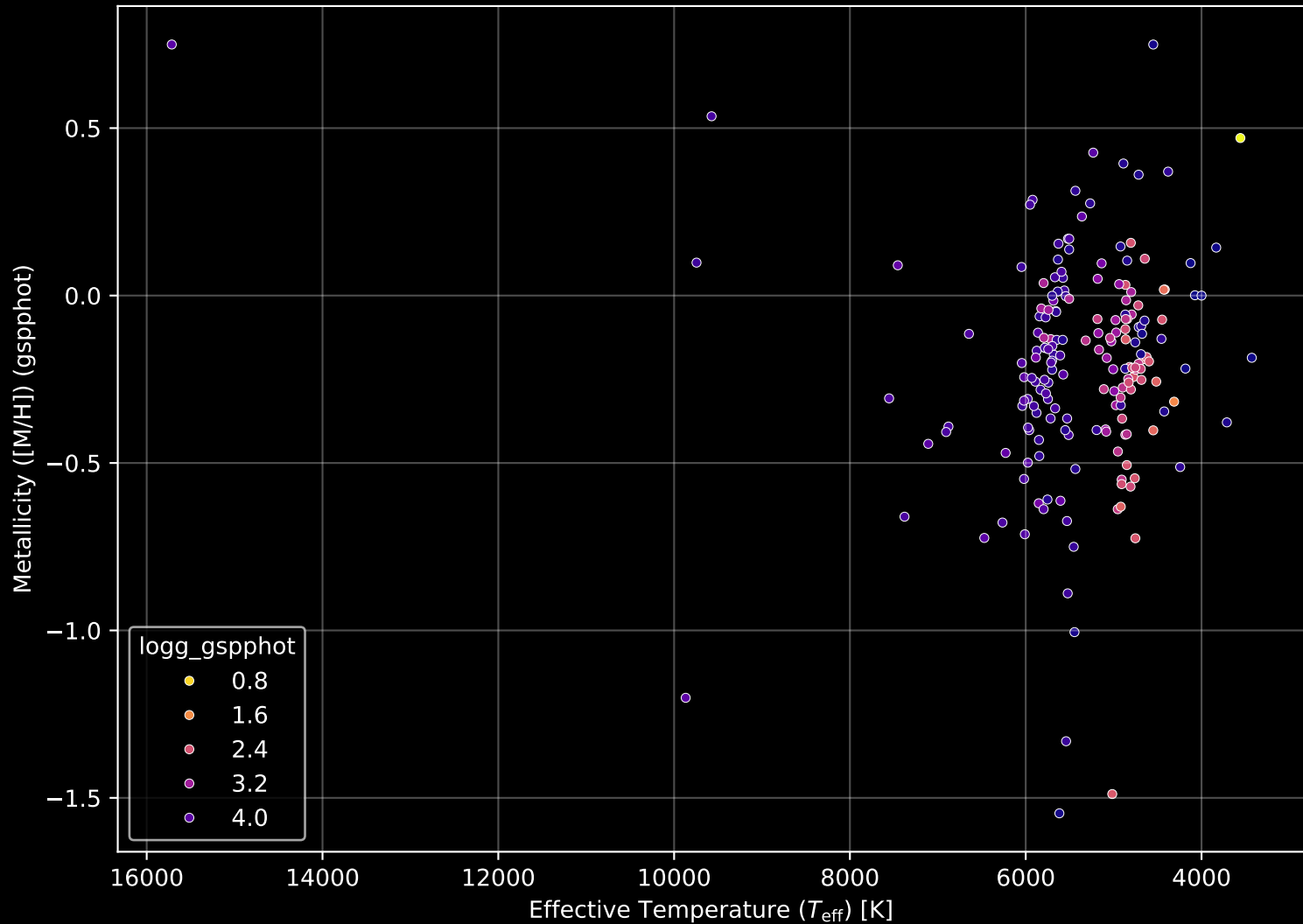
APOGEE DR17 Field: [269-28-O_TESS] Stellar Population Parameters (n= 187)
