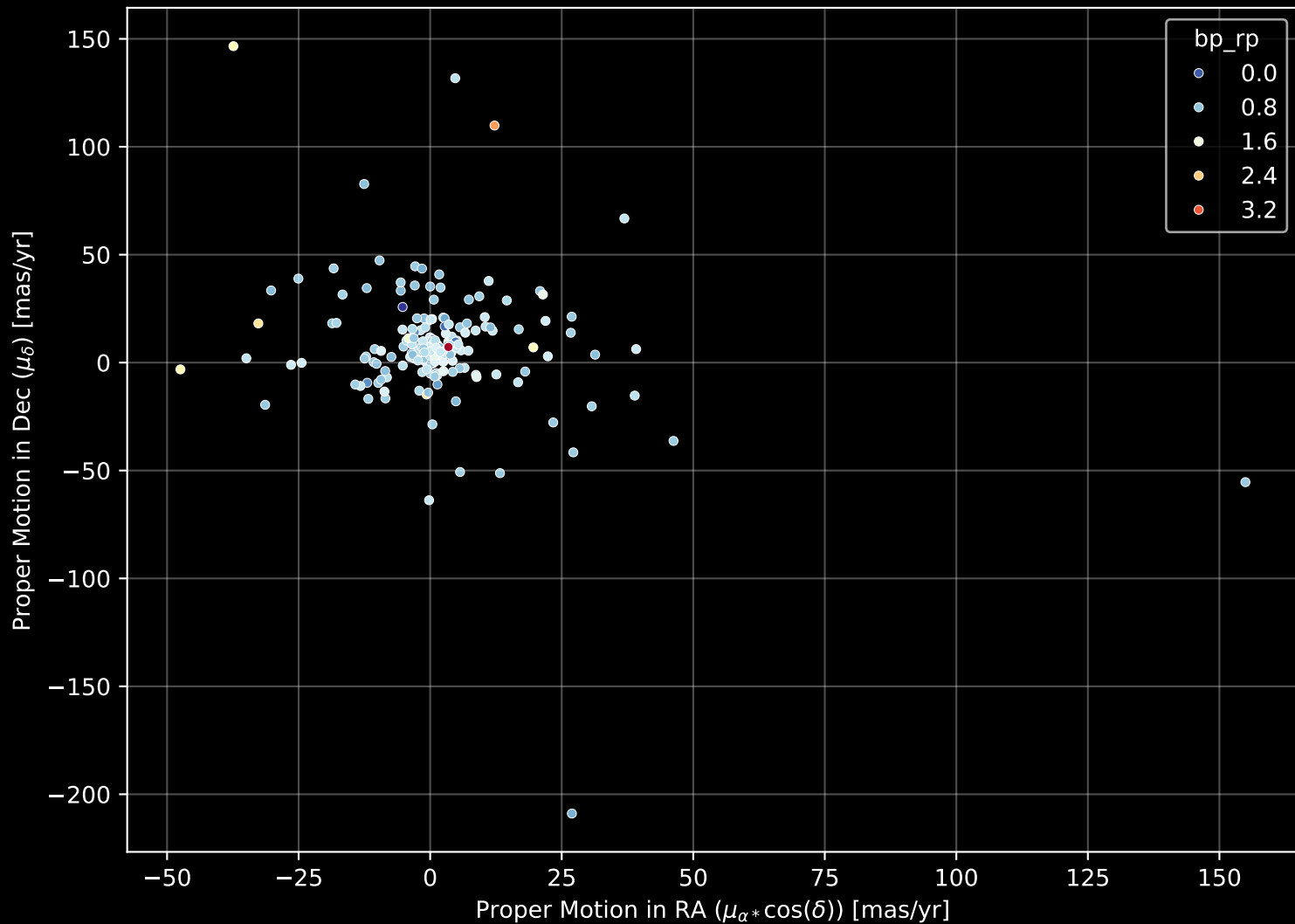
APOGEE DR17 Field: [269-28-O_TESS] Proper Motion Diagram (n= 187)
