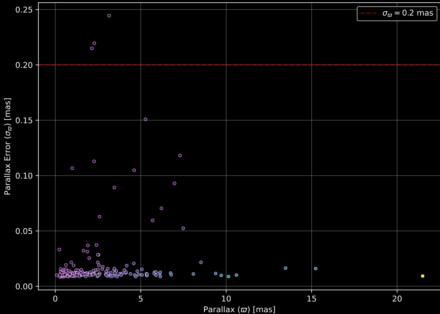
APOGEE DR17 Field: [269-28-O_TESS] Parallax Quality (n= 187)
