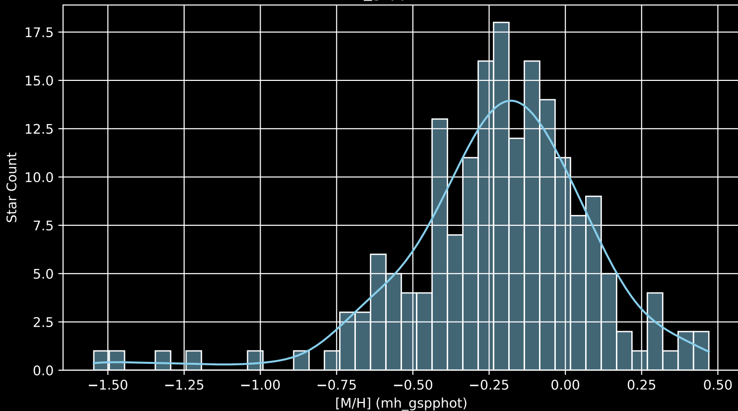
APOGEE DR17 Field: [269-28-O_TESS [M/H] (mh_gspphot) (n= 184)
