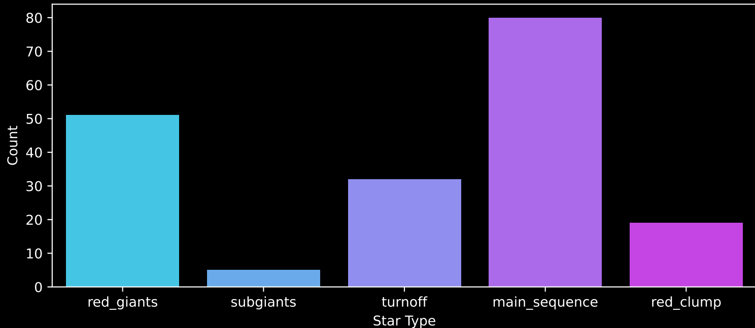
APOGEE DR17 Field: [269-28-O_TESS] Count plot of Star Type
