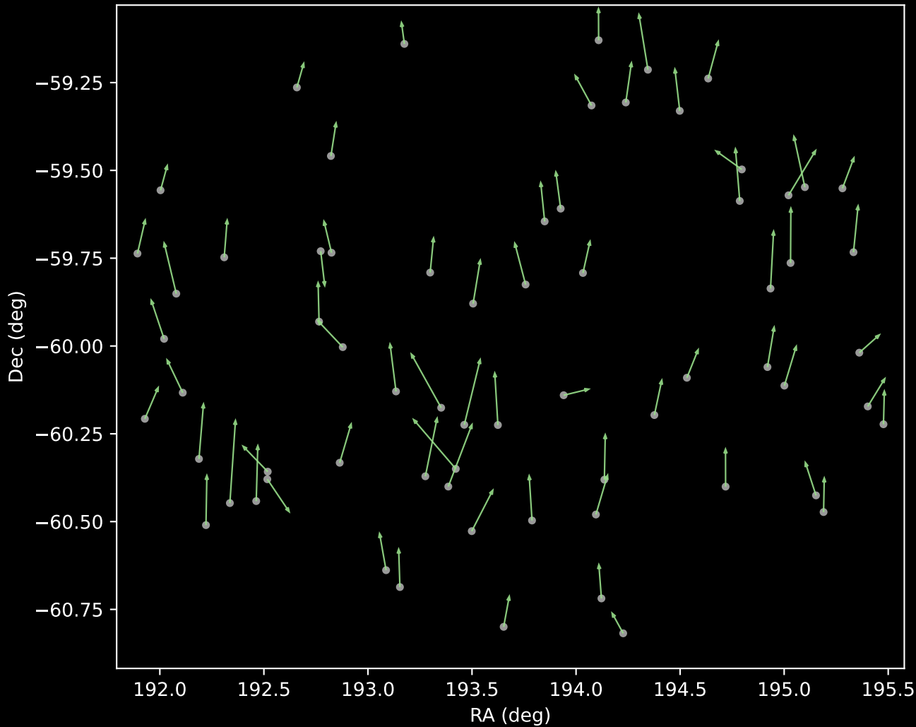
APOGEE DR17 Cluster 5 Proper Motion Vectors (n=68)
